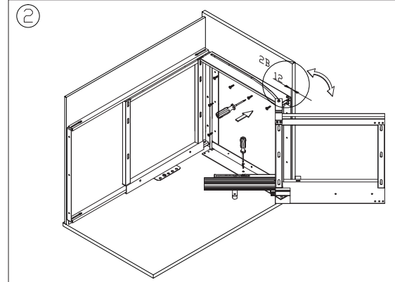
M3,5x16 SV/20
