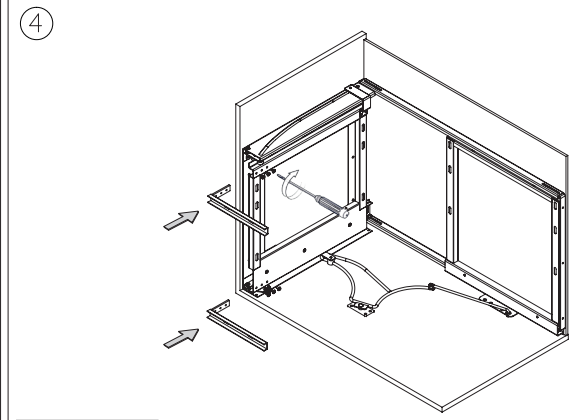
M5x10 RYSB/6
