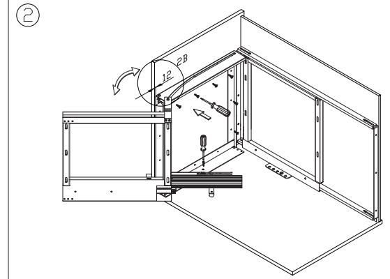
M3,5x16 SV/20
