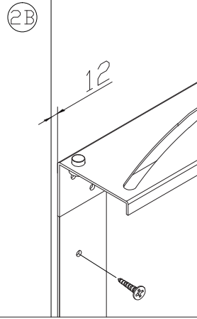
M3,5x16 SV/4
